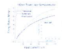
Fig. 5 Variation of frequency of spike with DC input current.
