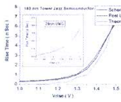
Fig. 6 Variation in rise time with rise time control signal V_{rise}
