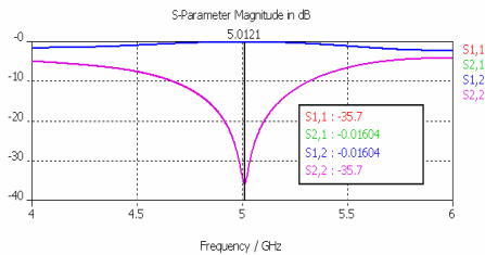
Figure 2. Plot of Return Loss & Insertion Loss
