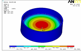
Figure 3. Temperature profile for loss 30.95 W
